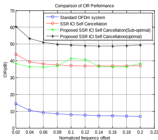
Fig 2.CIR versus Normalized frequency offset for various ICI cancellation schemes
