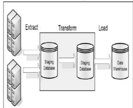
Figure 4. ETL process [4]
