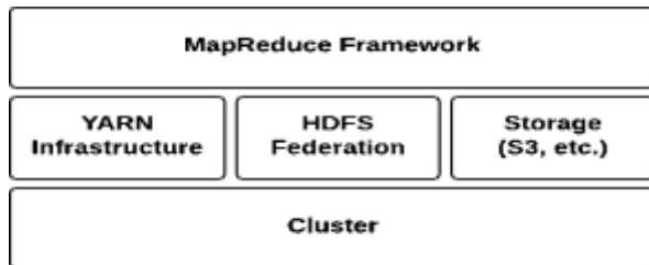
Figure 7. Hadoop Architecture
